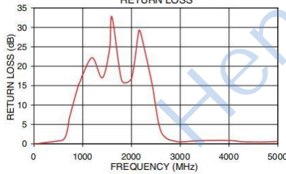
SXBP-1430-75+ RETURN LOSS
